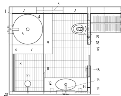
Bathroom floor plan
